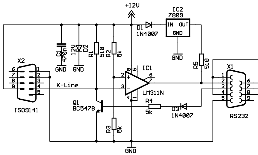
OBD-II ISO Interface for Vehicle Explorer www.obd-2.com
